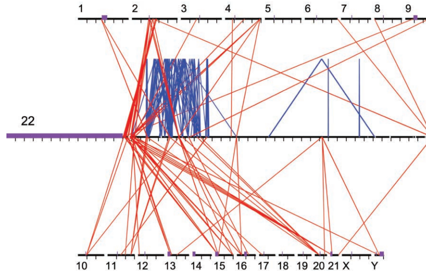
Figure 1 Spatial distribution of large segmental duplications between chromosome 22 and other human chromosomes. A scaled ( 50 \times ) version of chromosome 22, surrounded by the other chromosomes, shows lines representing interchromosomal ( red ) and intrachromosomal ( blue ) alignments ( \geq 10 kb). The majority of chromosome 22 pericentromeric duplications localize to the pericentromeric regions of other chromosomes. Likewise, the majority of subtelomeric duplications localize to subtelomeric regions of nonhomologous chromosomes. There is little cross-hybridization between subtelomeric and pericentromeric duplications. Chromosomes 2 and 20 share the largest amount of sequence with chromosome 22, whereas chromosomes 5, 7, 14, 18, 19, and X do not share any duplications with chromosome 22 that are >10 kb in size. The coordinates are based on the published UCSC human genome assembly. For chromosome 22, each tick mark represents a 1-Mb interval. For the other chromosomes, tick marks represent 50-Mb intervals. Purple boxes represent the unsequenced centromeres, acrocentric p arms, and Y heterochromatin. Gaps are denoted by white space. The program PARASIGHT was used to generate this diagram.
