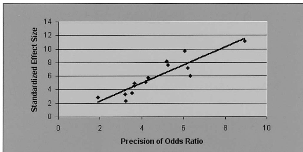
Figure 2 Regression of the standardized effect size versus the precision of the OR. The intercept of the line will occur close to 0, implying no bias in the samples.
