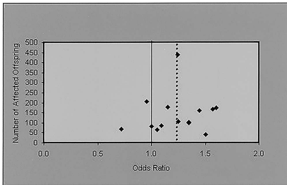
Figure 1 Funnel plot showing the number of affected offspring versus OR. The inverted funnel shape of this plot depicts results consistent with the absence of publication bias. The solid line represents OR = 1 , and the dotted line represents OR = 1.24 .
