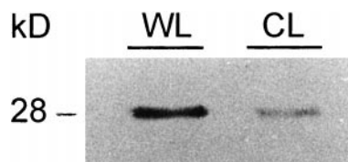
Figure 4. Protein gel-blot analysis of poplar protein extracts. Crude protein extracts from poplar control leaf (CL) and wounded leaf (WL) separated by SDS-PAGE, immobilized on a nitrocellulose membrane, and incubated with anti-CCoAOMT antibodies. The protein molecular mass is shown at the left in kD.
