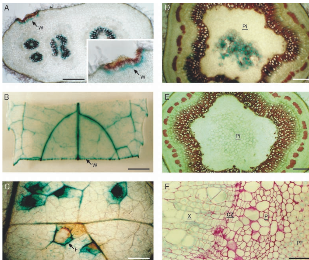
Figure 3. CCoAOMT promoter activity in transgenic poplar upon biotic and abiotic stress conditions. A, Transverse section of a petiole stained for both lignin and GUS. B, GUS activity in a mechanically wounded leaf. C, M. pinitorca -infected leaf stained for both lignin deposition and GUS activity. D, Double staining of a thick transverse section of a bent stem for lignin and GUS activity. E, Thick transverse section of a non-bent stem stained by P-HCl as control. F, Enlargement of a thin transverse section of the bent stem, transformed with PBINPOP1 . CZ, Cambial zone; F, site of fungal infection; P, phloem; PF, phloem fibers; Pi, pith; W, wound; X, xylem. Bars = 200 \mu m (in A, B, D, and E), 100 \mu m (in C), and 50 \mu m (in F).
