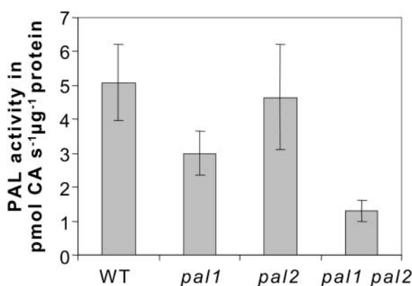
Figure 4. PAL Activity in 10-Week-Old Inflorescence Stems of the Wild Type and pal1 , pal2 , and pal1 pal2 Mutants.
