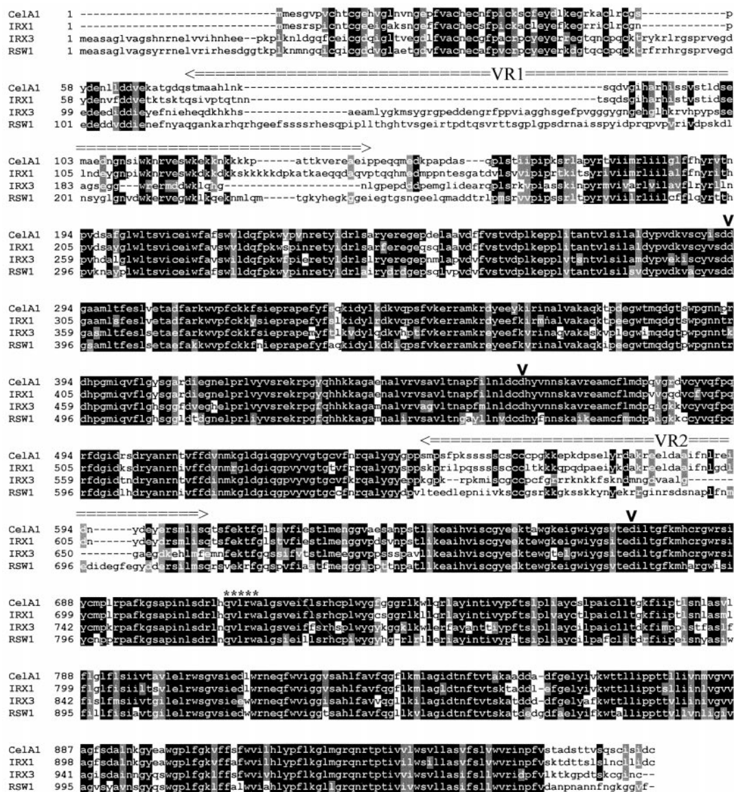
Figure 2. Alignment of the Amino Acid Sequences of Several Plant Cellulose Synthase Genes.
