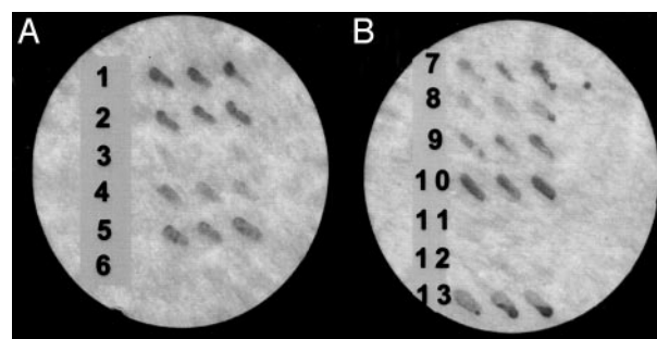
Fig. 3. One-on-one two-hybrid interactions. (A) GIPN interacts with RGS-GAIP (row 2), RGSZ1 (row 4), and RGSZ2 (row 5) but not with RGS4 (row 3) or RET-RGS1 (row 6). The interaction between RGS-GAIP and Gai3 (row 1) serves as positive control. (B) The N terminus of GIPN (amino acids 1–110) interacts with RGS-GAIP (row 7), RGSZ1 (row 8), and RGSZ2 (row 9). GIPN interacts with RGS-GAIP 1–79 (row 10) but not with RGS-GAIP 80–206 (row 11). RGS-GAIP 1–38 lacking the cysteine string motif does not interact with GIPN (row 12). RGS-GAIP 1–79 interacts with the N terminus of GIPN (amino acids 1–110) (row 13). Yeast were cotransformed with the indicated constructs. For each interaction pair, three separate colonies were streaked on a filter and scored for \beta -galactosidase activity.
