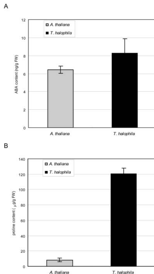
Figure 6. ABA and Pro contents in salt cress and Arabidopsis. A, Accumulation of ABA in the entire plant of salt cress and Arabidopsis during normal growth conditions in hydroponic culture. Three-week-old Arabidopsis and 4-week-old salt cress plants grown under normal conditions were used for the analysis. B, Pro content in the entire plant of salt cress and Arabidopsis during normal growth conditions in hydroponic culture. Three-week-old Arabidopsis and 4-week-old salt cress plants grown under normal conditions were used for the analysis.
