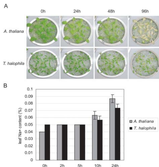
Figure 2. Evaluation of salt tolerance and Na + uptake in hydroponic culture system. A, High salinity stress tolerance in hydroponic culture system. Three-week-old Arabidopsis and 4-week-old salt cress plants that were the same in size were exposed to 250 mM NaCl solution for 24, 48, and 96 h. B, Accumulation of NaCl in leaves of Arabidopsis and salt cress during high salt stress in hydroponic culture system. Three-week-old Arabidopsis and 4-week-old salt cress plants that were the same size were exposed to 250 mM NaCl solution for 2, 5, 10, and 24 h.
