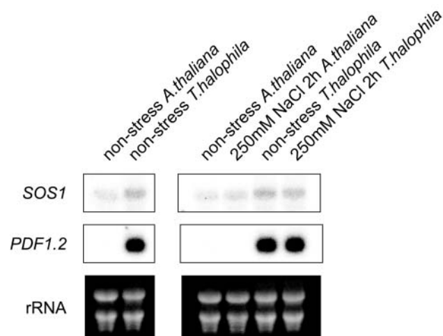
Figure 5. RNA gel-blot analysis of AtP5CS , ThP5CS , SOS1 , and PDF1.2 genes in salt cress and Arabidopsis. Total RNA was prepared from 3-week-old Arabidopsis and 4-week-old salt cress plants that were the same in size during nonstress or 250 mM NaCl stress using the microarray analyses. Each lane was loaded with 10 \mu g of total RNA. The RNA was fractionated on a 1% agarose gel, blotted onto a nylon membrane, and hybridized with ^{32} P-labeled AtP5CS , ThP5CS , SOS1 , and PDF1.2 DNA fragments as probes.
