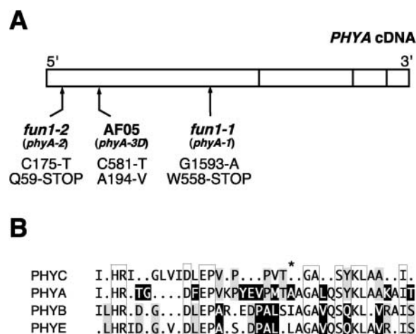
Figure 5. Molecular lesions in pea phyA mutants. A, Location and nature of mutations in the pea PHYA cDNA. B, Alignment of consensus amino acid sequences for each phytochrome type in the region surrounding the residue substituted in the phyA-3D mutant (A194; marked with asterisk). These consensus sequences are derived from alignments of all available full-length dicot sequences for each phytochrome type and show only residues that are invariant for each phytochrome type. This region spans amino acids 170 to 209 in the pea PHYA apoprotein, which correspond to positions 219 to 259 in the alignment of Mathews et al. (1995). Residues perfectly conserved across all full-length sequences are boxed. Residues perfectly conserved and uniquely present in phyA or phyB/E are shown in black. Other residues perfectly conserved in phyA or phyB/E are shaded.
