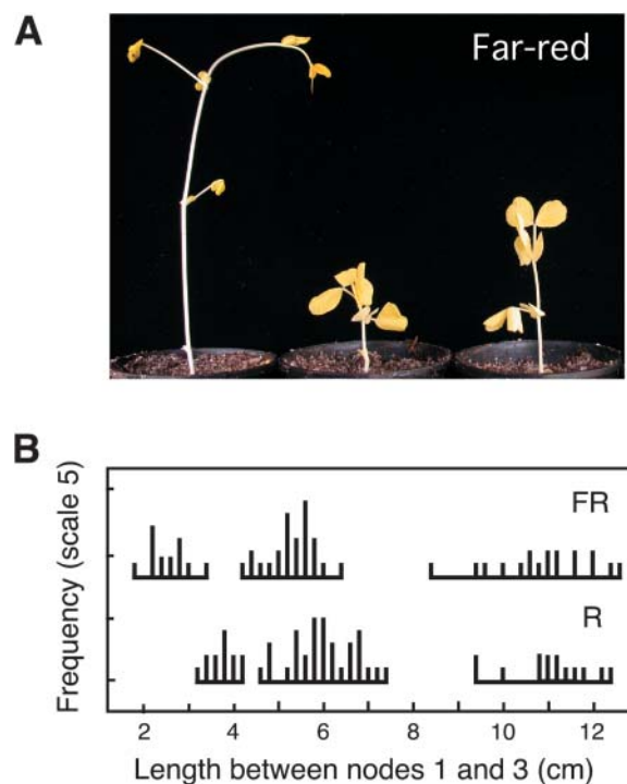
Figure 1. Inheritance of the enhanced response to FR in the AF05 mutant. A, Twelve-day-old wild-type, homozygous AF05 mutant, and cop1-1 mutant seedlings grown from sowing under continuous FR ( 10 \mu\text{mol m}^{-2} \text{s}^{-1} ). B, Segregation for internode length in the F_2 progeny of a cross between AF05 and wild-type cv Torsdag grown under continuous FR or R.
