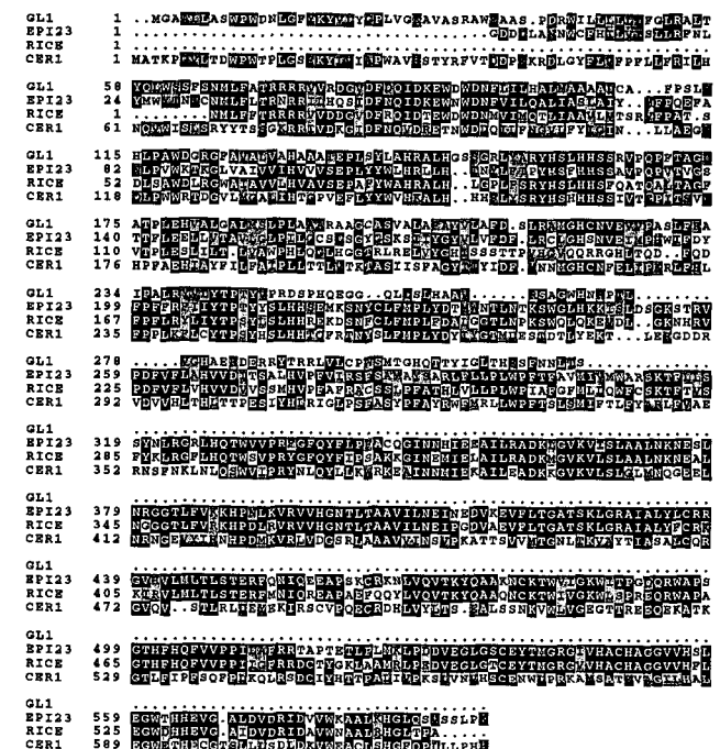
Figure 4. Comparison of the deduced amino acid sequences of the proteins coded by maize gl1 (GL1), K. odora epi23 (EPI23), Arabidopsis CER1 (CER1), and the rice EST RICS2751A (RICE). Identical residues are boxed in black; conservative substitutions are boxed in gray. Dots represent gaps that were inserted to maximize the alignment.
