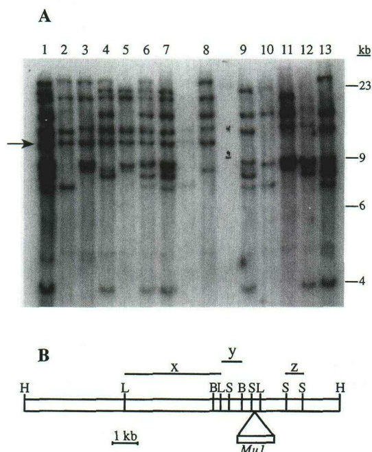
Figure 2. Identification of a Mu1 -containing 12.5-kb Hind III DNA fragment that co-segregates with the gl1 -755048 allele. A, Southern blot of Hind III-digested maize DNA probed with a Mu1 -specific probe. The arrow indicates the 12.5-kb DNA fragment, which is present in all plants carrying the gl1 -755048 allele and absent in sibling plants that do not carry this allele. Lanes 1 through 8, DNA from individual plants of genotype gl1 -755048/ G1 ; lanes 9 through 13, DNA from individual plants of genotype G1 / G1 . B, Restriction map of the 12.5-kb Mu1 -containing Hind III insert from \lambda 1211. DNA fragments x, y, and z were used as the probes in later analyses. H, Hind III; L, Sal I; B, Bam HI; and S, Sac I.
