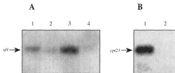
Figure 5. A, Effects of mutations at the gl1 locus on GL1 mRNA accumulation. Northern blot of RNA from seedlings of the maize inbred B73 (lanes 1 and 2) and standard Q60 (lanes 3 and 4). These seedlings were homozygous at the gl1 locus for wild-type Gl1 ( Gl1 +B73, lane 1; Gl1 +Q60, lane 3) or mutant ( gl1-ref , lane 2; gl1-755048 , lane 4) alleles. B, Epidermis-specific accumulation of epi23 mRNA. Northern blot of RNA from epidermal (lane 1) or nonepidermal (lane 2) tissues of K. odora .
