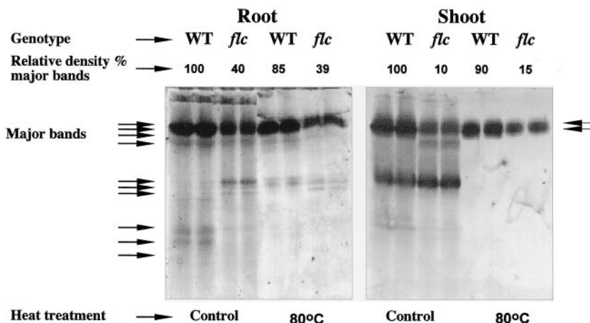
Figure 2. Immunoblot analysis of MoCo-containing hydroxylases. Approximately 200 \mu g of total soluble protein from root and shoot extracts were fractionated on native-PAGE and examined with anti-TAO1 antibodies. Untreated (Control) and preheated (80°C for 90 s) treatments were used. flc , flacca tomato genotype.
