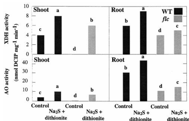
Figure 4. AO and XDH activities of shoot and root extracts of the WT and flacca ( flc ) genotypes. Extracts were assayed in vitro with hypoxanthine and indole-3-aldehyde as the substrates. The assays were carried out with desalted extracts, with or without preincubation with \text{Na}_2\text{S} and dithionite. Enzyme activities are expressed as nmol DCIP \text{mg}^{-1} \text{min}^{-1} . Lowercase letters indicate statistical significance of the separation between treatments carried out by the multiple range test (Duncan test; P < 0.05 , n = 5 ). The data represent one of three different experiments that yielded essentially identical results.
