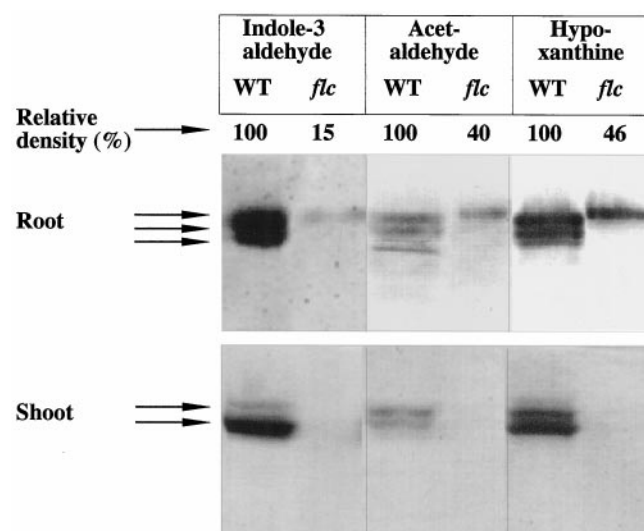
Figure 1. Native-PAGE of shoot and root extracts of WT and flacca ( flc ) tomato genotypes showing AO and XDH activities. Activity gels were loaded with 300 \mu\text{g} of soluble protein of the crude extract of shoots or 100 \mu\text{g} of soluble protein of roots and stained with the appropriate substrate as described in "Materials and Methods."
