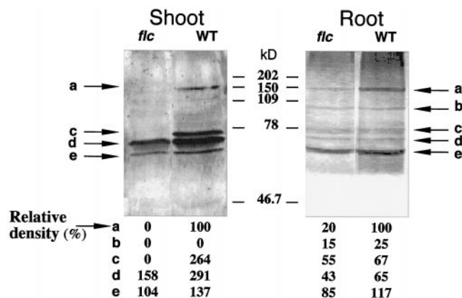
Figure 3. Immunoblot analysis of MoCo-containing hydroxylases. Crude extracts of roots and shoots of WT and flacca ( flc ) tomato plants were fractionated on SDS-PAGE. The gel was loaded with approximately 50 \mu g of total soluble protein and examined with anti-TAO1 antibodies. Relative density measurements of the bands are indicated at the bottom of the panels.
