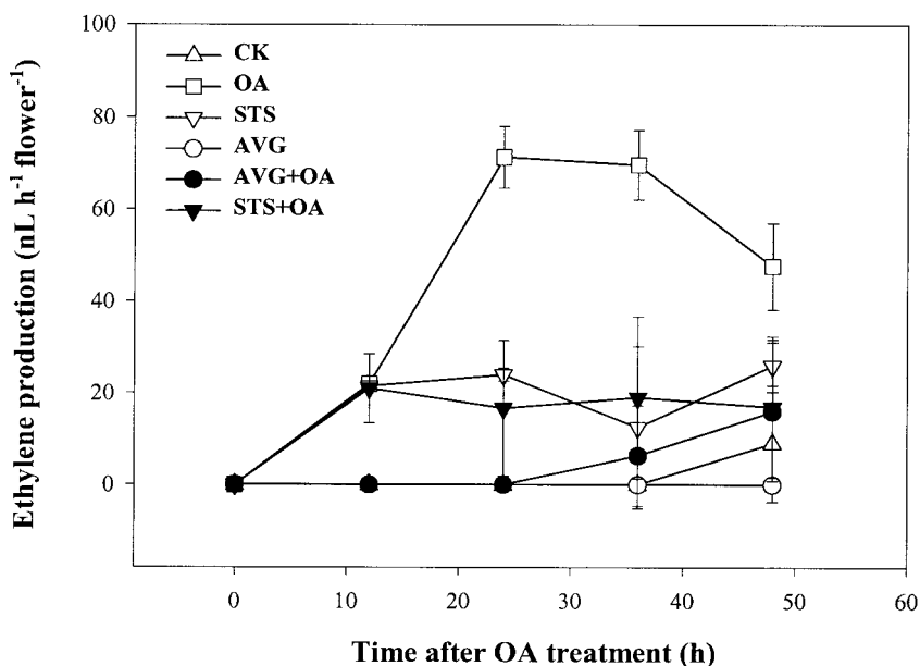
Figure 3. Effects of AVG and STS treatments on the OA-induced ethylene production. Twenty microliters of solution containing 0.8 nmol AVG or 2 nmol STS, where indicated, was applied to the stigma 12 h prior to the OA treatment. Ethylene was measured as in Figure 2.
