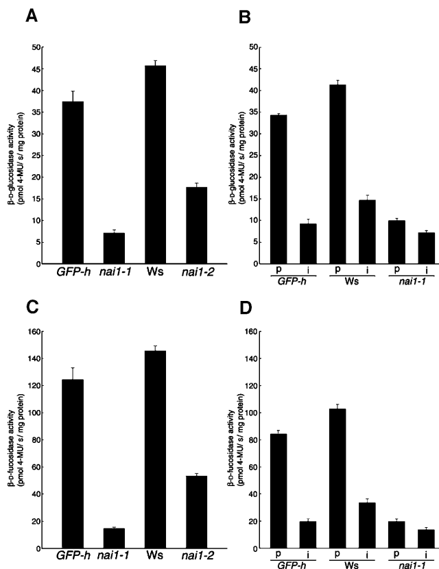
Figure 7. Decreased β-D-Glucosidase and β-D-Fucosidase Activity in nai1-1 and nai1-2 Mutants.
