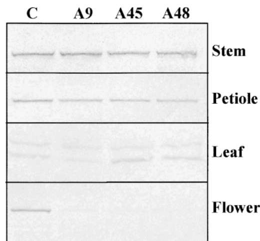
Figure 2. Protein Gel Blot Analysis of SuSy in Different Tissues from Control and Transgenic Lines.
