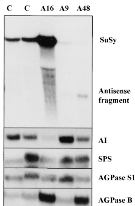
Figure 3. RNA Gel Blot Analysis of Carbon Metabolism in SuSy Antisense Tomato Fruits.
