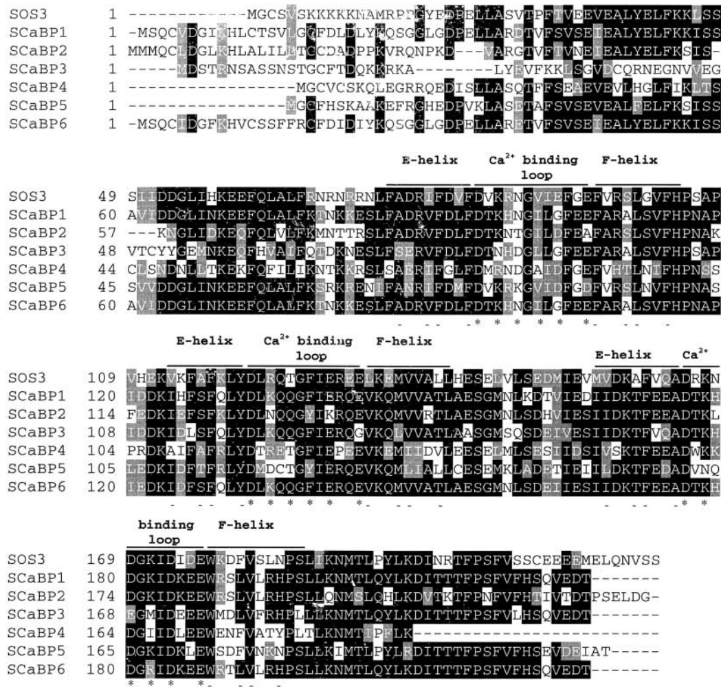
Figure 5. Alignment of SOS3 with SCA1Ps.
