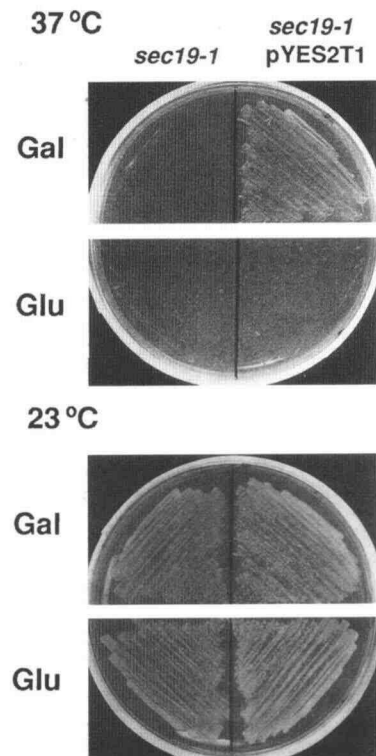
Figure 7. AtGDI1 Complements the Yeast sec19-1 Mutant.
