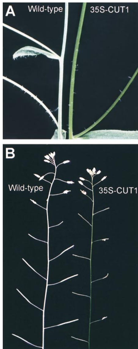
Figure 5. 35S- CUT1 Plants Display a Waxless Phenotype and Are Male Sterile.
